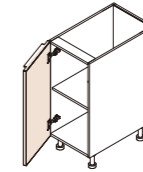
Item: Vanity Base With 1 Door Code: VB15FD, VB18FD, VB21FD HxD: 30" x 21"
