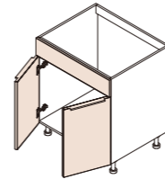
Item: Vanity Sink Base With 2 Doors+1 Fake Drawer Code: VSB24, VSB27, VSB30, VSB36 HxD: 30" x 21"
