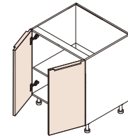
Item: Vanity Base With 2 Doors Code: VB24FD, VB30FD, VB36FD HxD: 30" x 21"
