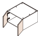
Item: Wall Cabinet For Fridge Code: W301224, W361224, W301524 W361524, W301824, W361824 W302124, W362124 HxD: 12/15/18/21" x 24"
