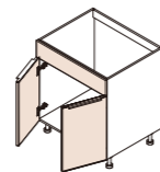
Item: Sink Base Cabinet Code: SB30, SB33, SB36, SB42 HxD: 30" x 24"
